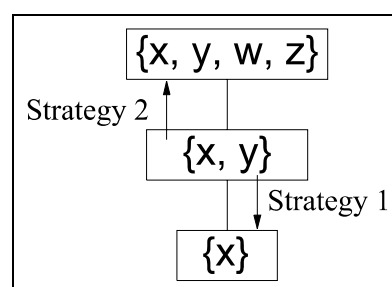
Figure 1 Illustration of two treatment strategies. Strategy 1 tries to remove HIV entirely from the system. Strategy 2 aims at establishing a long-term CTL-mediated control of viral load.
