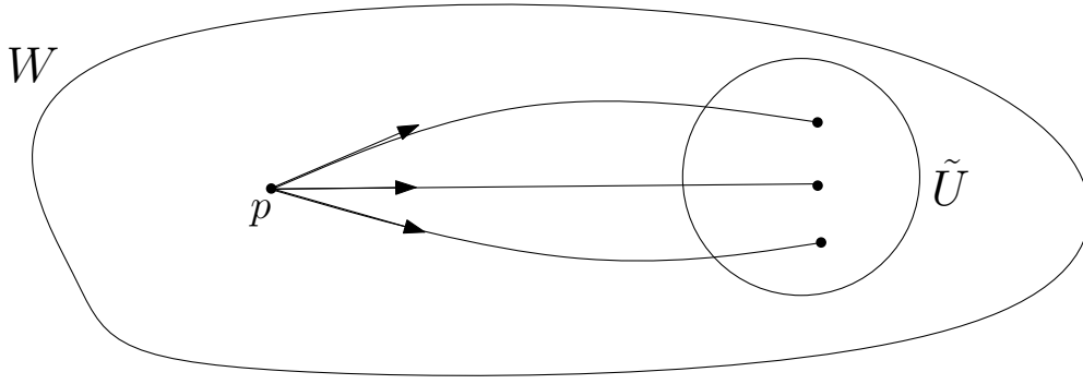
FIGURE 2. \bar{\lambda}^i at p is orthogonal to every \hat{\gamma}_{p,\bar{p}}^i , implying \lambda^i \equiv 0 .
