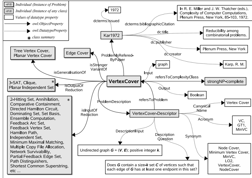
Figure 2: The VERTEX COVER Decision Problem and its Relationships.
