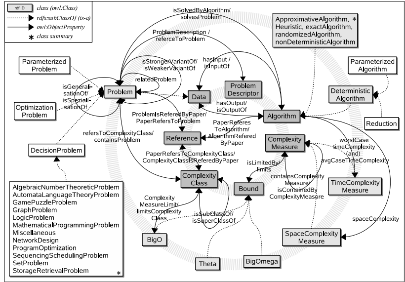
Figure 1: Simplified Ontology for NP-complete problems covering only the most important classes and their relationships.
