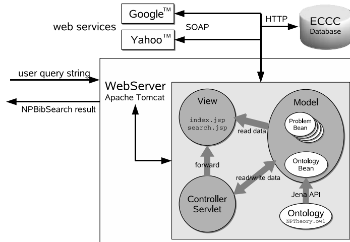
Figure 3: Schematic Overview of the NPBibSearch Architecture.
